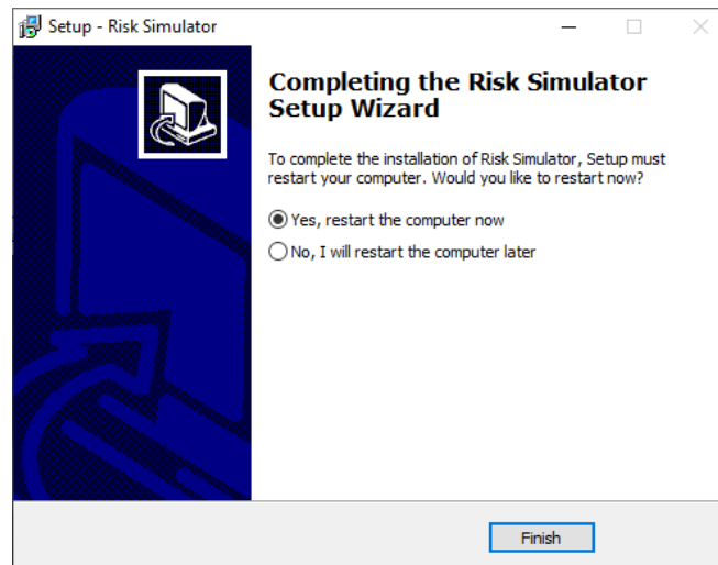
Figura 14. Finish
